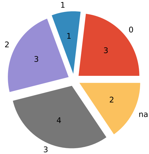
Rep (total=13)
