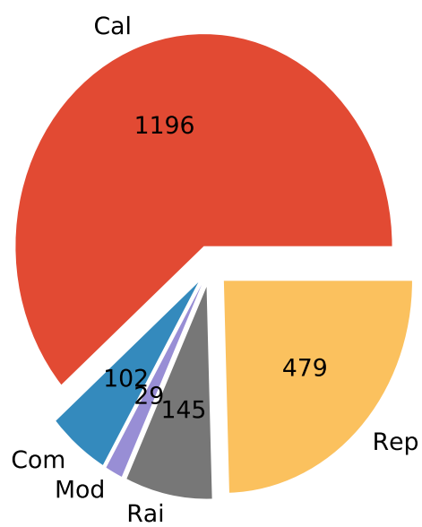
sum (total=1950.0)
