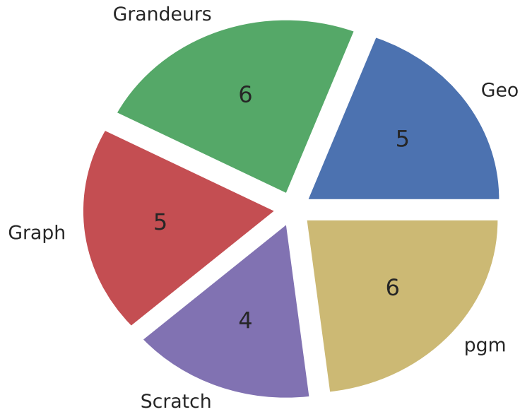
sum (total=26)
