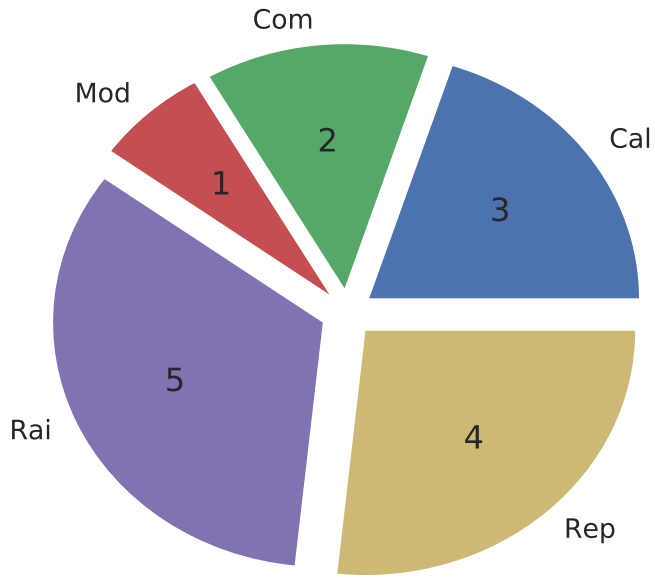
sum (total=15)
