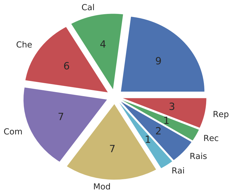
sum (total=39.0)
