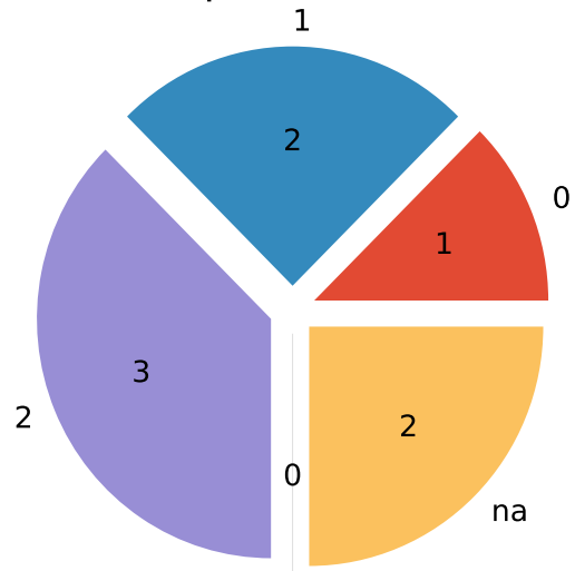
Rep (total=8)
