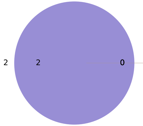
Com (total=2)
