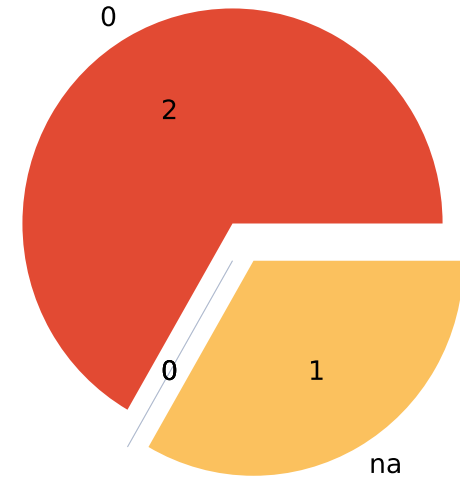
Rai (total=3)
