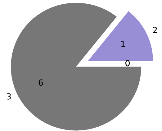
Prop (total=7)
