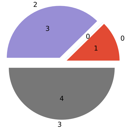
Tria (total=8)
