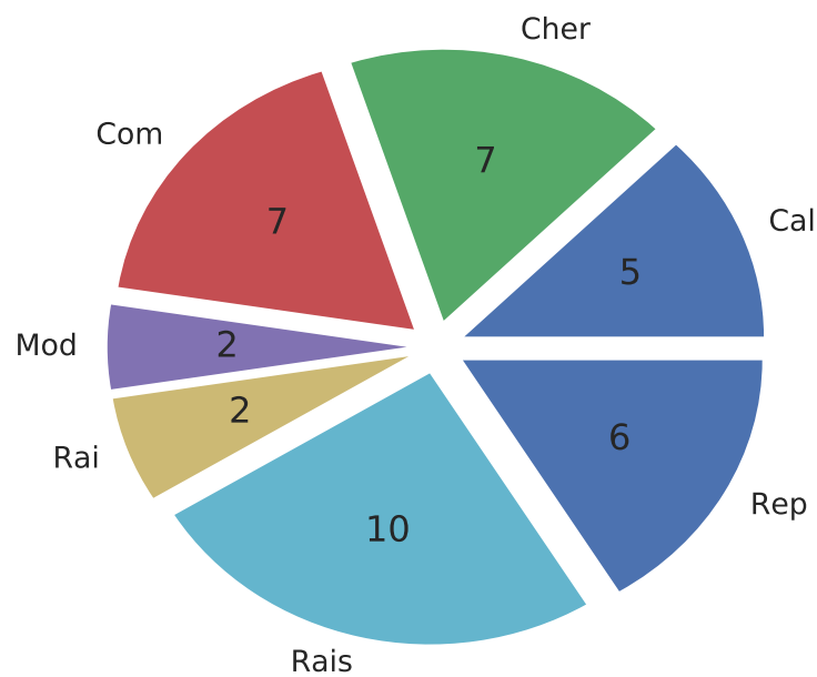
sum (total=40.0)
