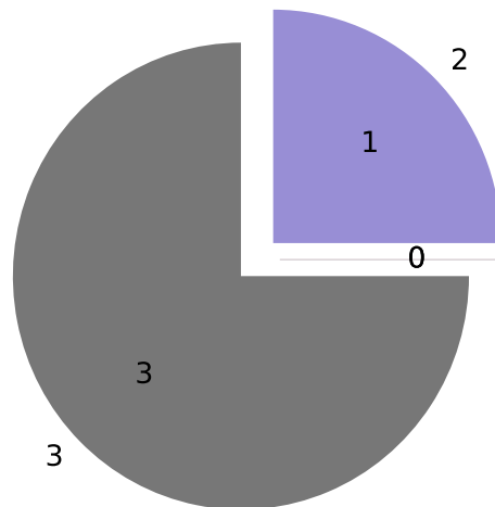
Com (total=4)
