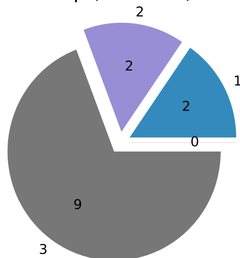
Rep (total=13)
