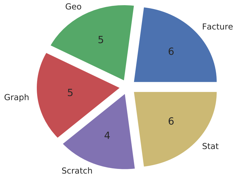
sum (total=26)
