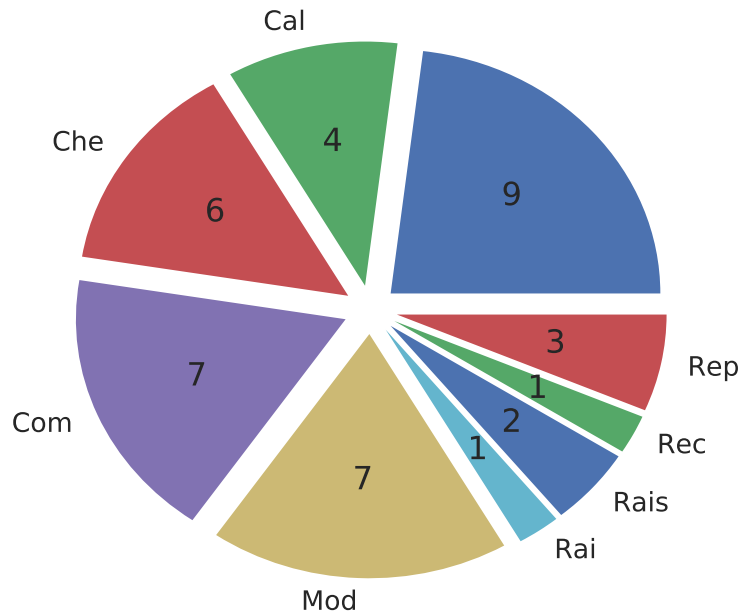
sum (total=39.0)
