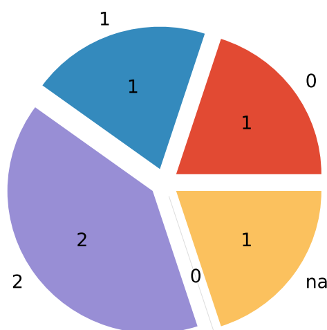
Tria (total=5)
