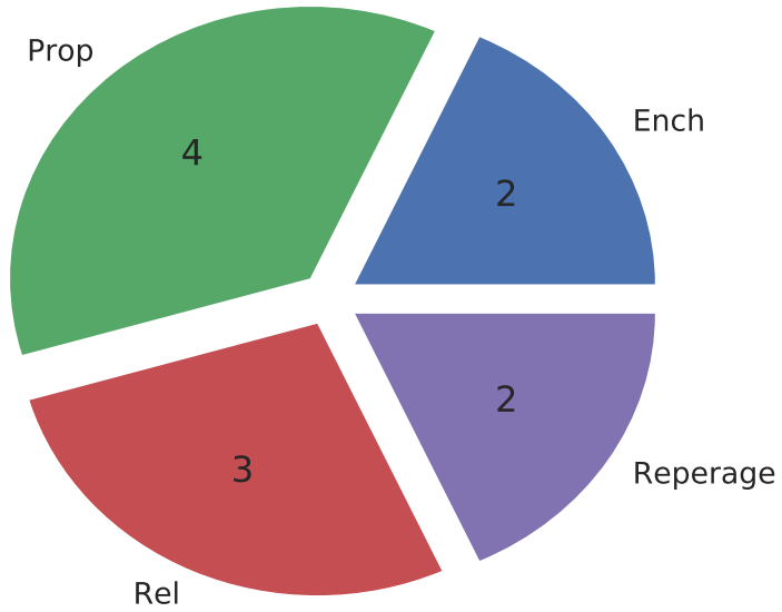
sum (total=11)
